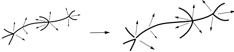
FIGURE 2. Diffeomorphism of a Skeletal Structure
