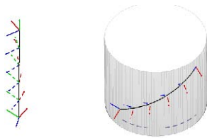
Figure 3. Three-dimensional rotational-flows interpolation. x_t lies on a helix whose axis is the axis of rotation between E_0 and E_1 .
