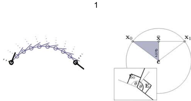
Figure 1. (Left) Examples of planar points: x_0 and x_1 and the corresponding frames: E_0 and E_1 . The solid line indicates the e_{0,t} basis direction, and the dotted line indicates e_{1,t} . The interpolation provided by our method is indicated by a lighter color. Note that the frame rotates concurrently with the point. (Center) The geometry of rotational-flows interpolation in two dimensions. The rotation required to bring E_0 onto E_1 (inset) defines the angle \theta swept out by the interpolating path from x_0 to x_1 . The path lies on a circle whose geometry can be derived from the positions of the points and the angle \theta . (Right) The point x_t is reached after interpolating t fraction of the way from x_0 to x_1 . If we then interpolate from x_t to x_1 our method continues along the original circular arc.
