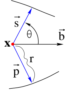
Fig. 2. A medial atom with its implied boundary
